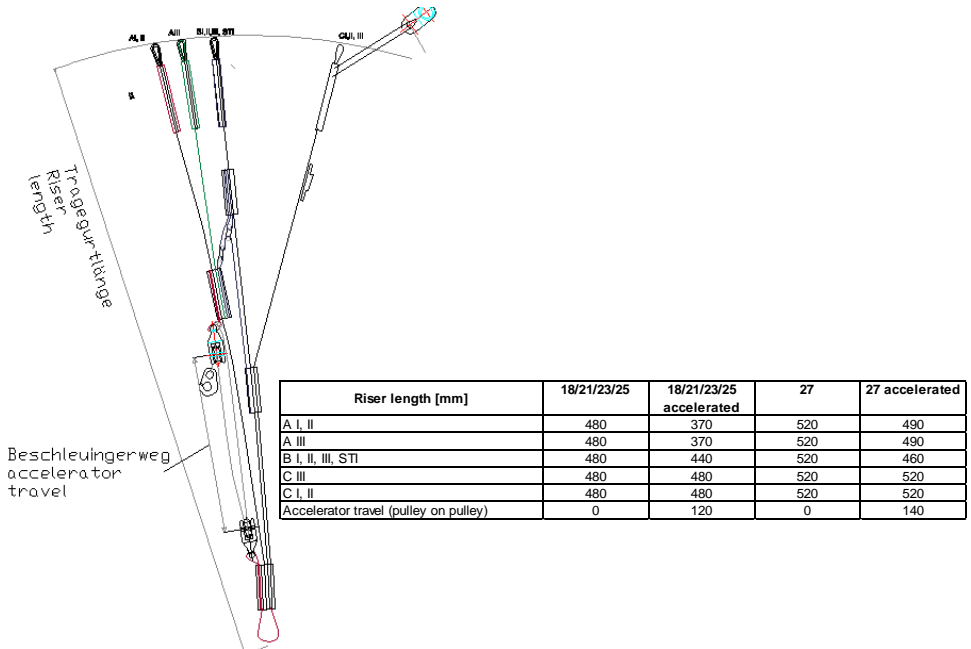
Illustration 3: UP Mana riser
