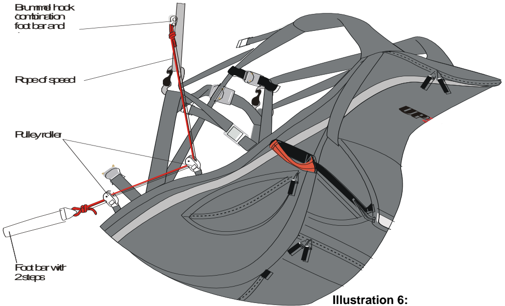
Illustration 6: Harness with speed system
