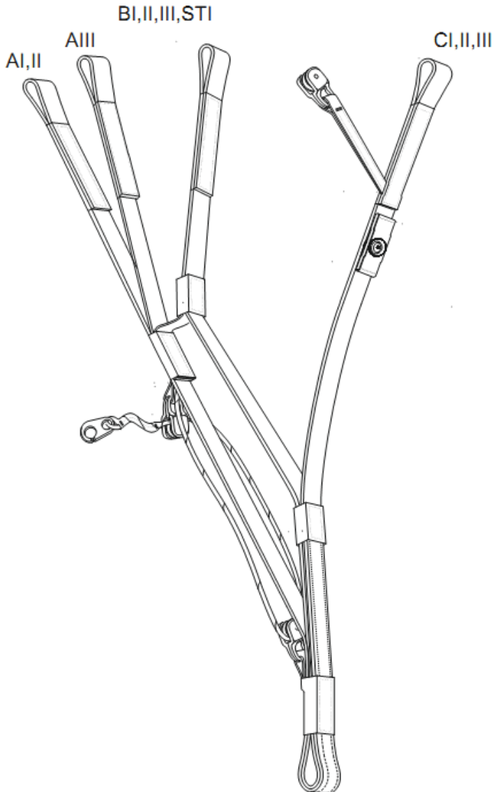
Illustration 2: UP Makalu 3 riser
